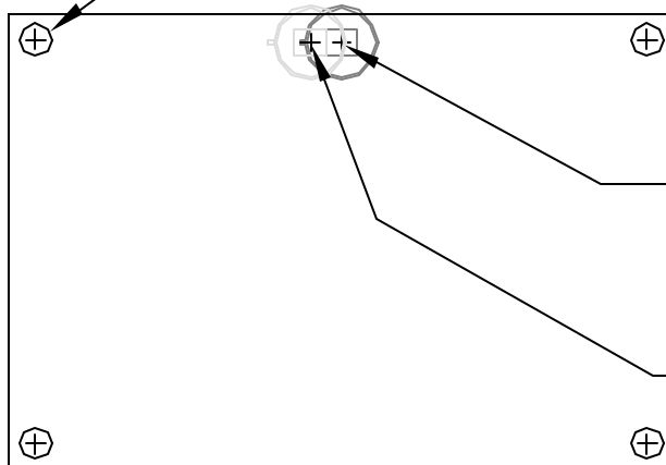
CIRCUIT BOARD MOUNTING TEMPLATE
