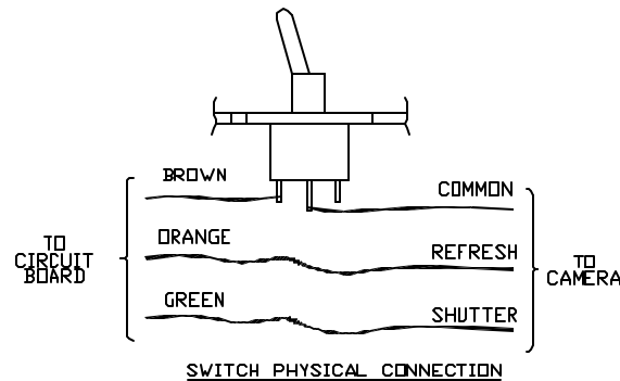
TYPICAL CAMERA CONNECTION AND INHIBIT SWITCH
